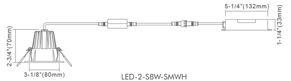
LED-2-S8W-SMWH
