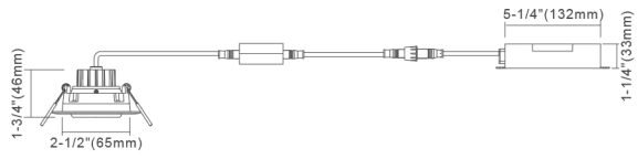
AD-LED-3-S8W-SMWH-EY
