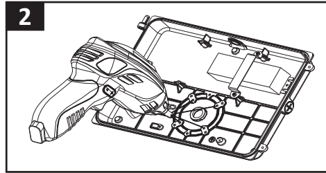
Remove the Housing Back Plate and unscrew center Plug, using a drill open installation holes in Housing Back Plate.
