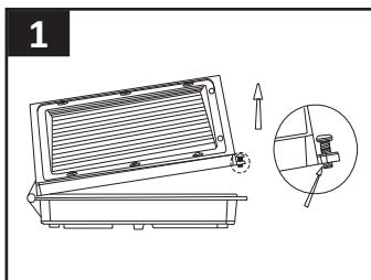
Using a screwdriver loosen side Housing Screws.
