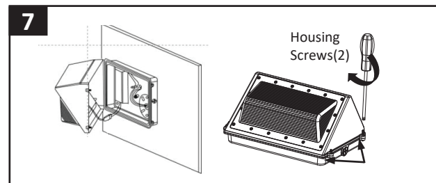
Make connections LED Driver to LED Modules and Mount the Housing over the Housing Back Plate and secure with (2) Screws (provided).
