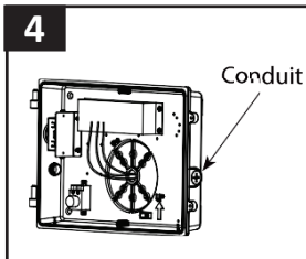
Feed supply wires through Housing Back Plate center Plug. Connect Wiring.
