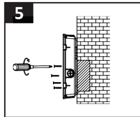
Secure Housing Back Plate to surface or junction box with Screws (supplied by others).
